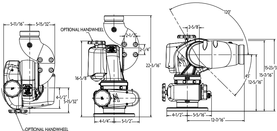
Style 1578 SaberMaster Nozzle
